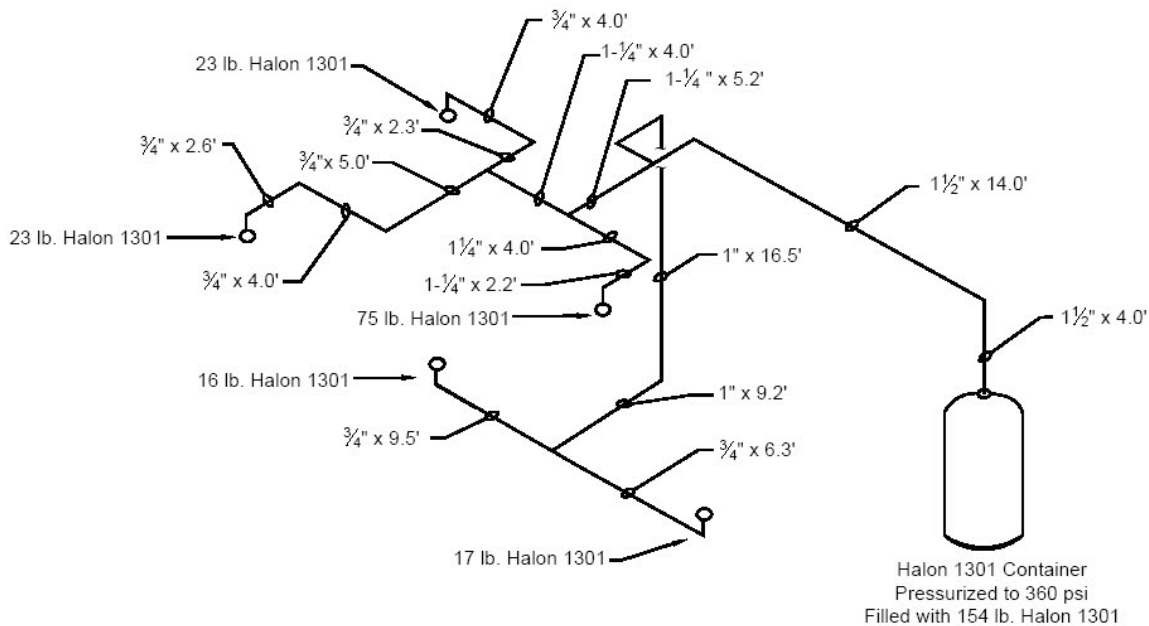
Halon Piping Isometric
