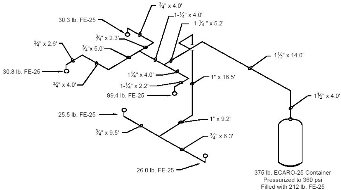
ECARO-25 Piping Isometric
